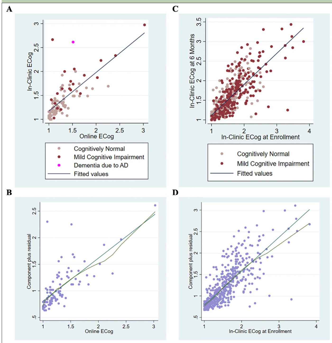
Figure 2. Scatterplots and Component Plus Residual Plots of Everyday Cognition Total Scores
